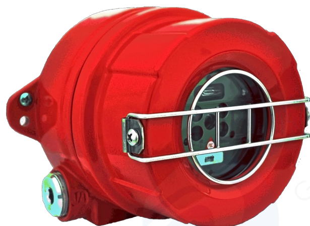
Standard Model
