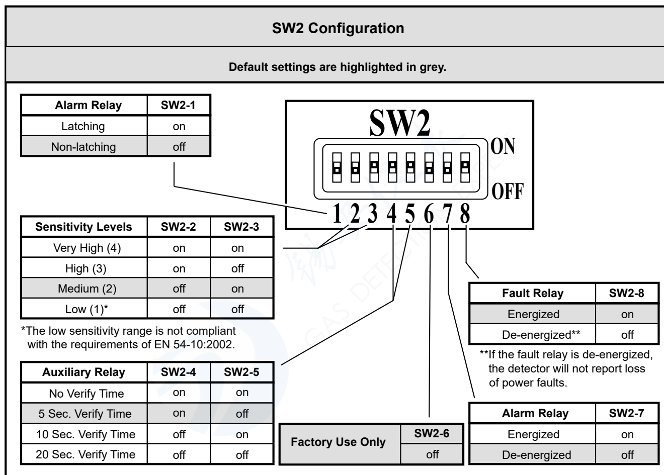
Figure 25. Eight-position DIP switch SW2
